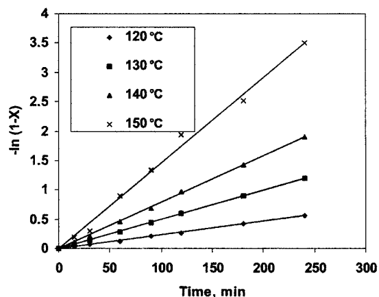
Figure 11. Plot of -\ln(1-X) vs time at different temperatures.
