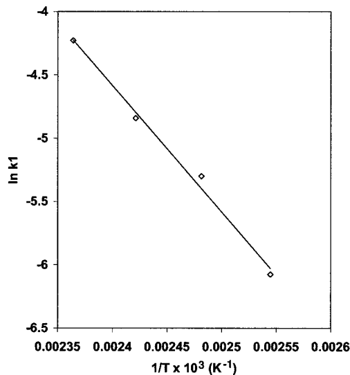
Figure 12. Arrhenius plot.
