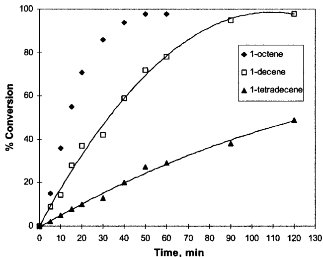
Figure 14. Alkylation of benzene with different olefins. Olefin: benzene, 1:10 mol; temperature, 150 °C; catalyst load, 0.05 g/mL; rpm, 1000; reaction time 2 h.
