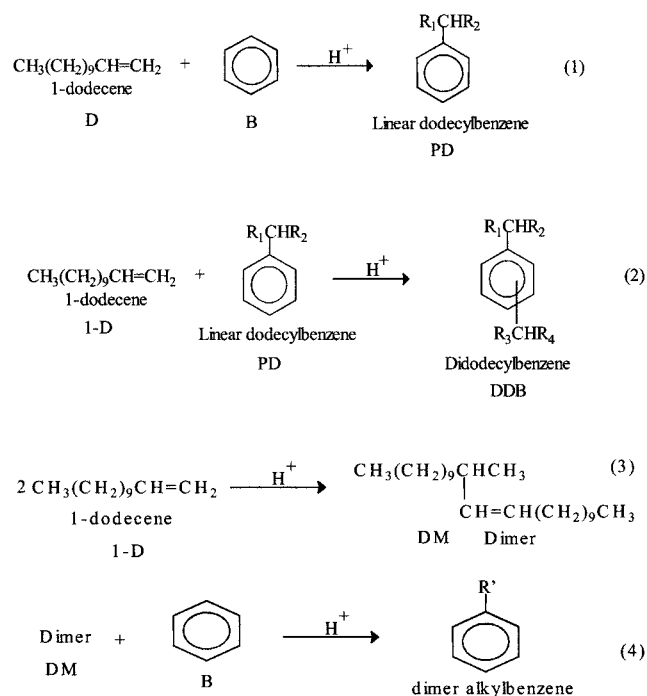
Scheme 1. Possible series and parallel reactions during alkylation of benzene with 1-dodecene
