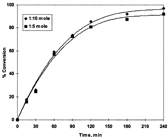
Figure 4. Effect of mol ratio on benzene alkylation with 1-dodecene. Catalyst DTP/K-10, 0.05 g/mL, temperature, 150 °C; speed, 1000 rpm; reaction time, 4 h.
