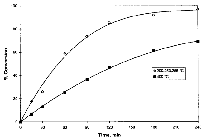
Figure 2. Effect of calcination temperature on benzene alkylation with 1-dodecene. C 12 :C 6 H 6 , 1:10 mol; catalyst DTP/K-10, 0.05 g/mL; temperature, 150 °C; speed, 1000 rpm; reaction time, 4 h.
