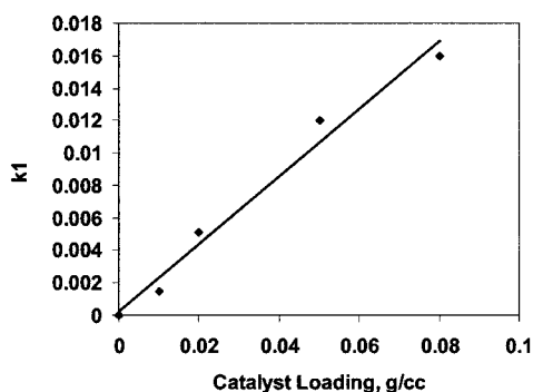
Figure 9. Plot of k_1 vs catalyst loading.
