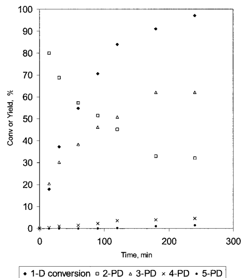
Figure 1. Alkylation of benzene with 1-dodecene over 20% DTP/K-10. Distribution of linear phenyldodecanes in the reaction mixture. Reaction conditions: benzene:1-dodecene = 10:1, 150 °C, 1000 rpm, autoclaved. 20% DTP/K-10 catalyst loading: 0.05 g/mL.
