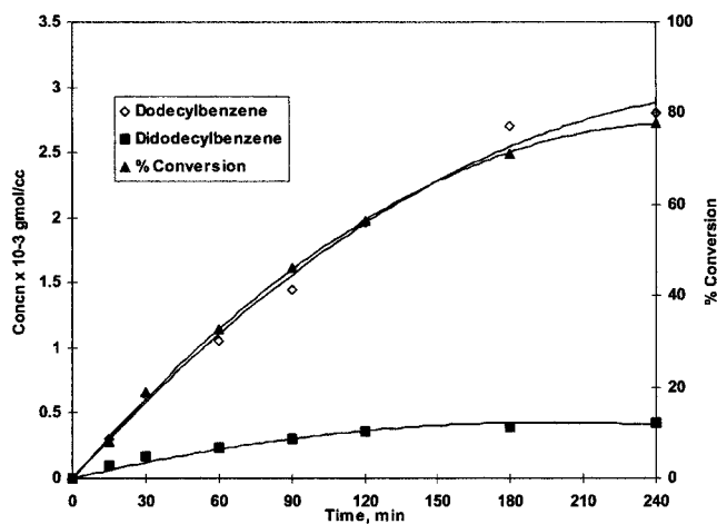
Figure 5. Effect of mol ratio on yields of mono- and dialkylated products in benzene alkylation with 1-dodecene. C 12 :C 6 H 6 , 1:2 mol; catalyst DTP/K-10, 0.05 g/mL, temperature, 150 °C; speed, 1000 rpm; reaction time, 4 h.
