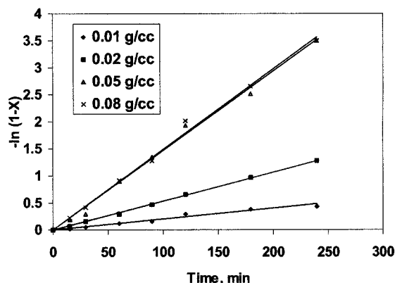
Figure 8. Plot of -\ln(1-X) vs time at different catalyst loading.
